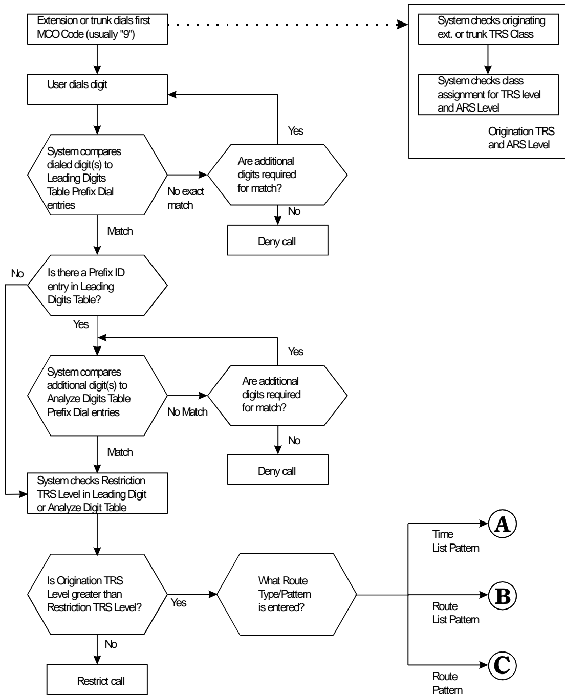
Figure A-2. ARS/TRS Flowchart Page 1 of 2
