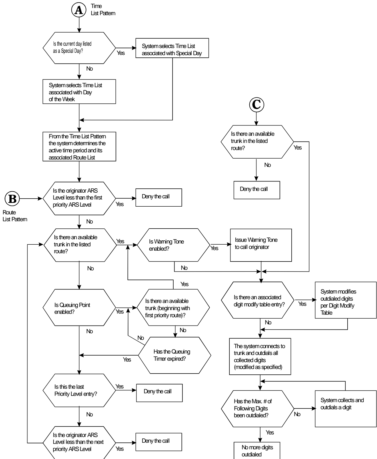
Figure A-3. ARS/TRS Flowchart Page 2 of 2
