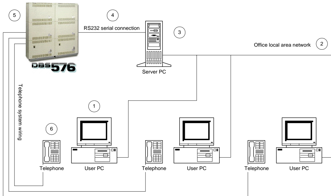
Figure 3-1. LAN TAPI system
